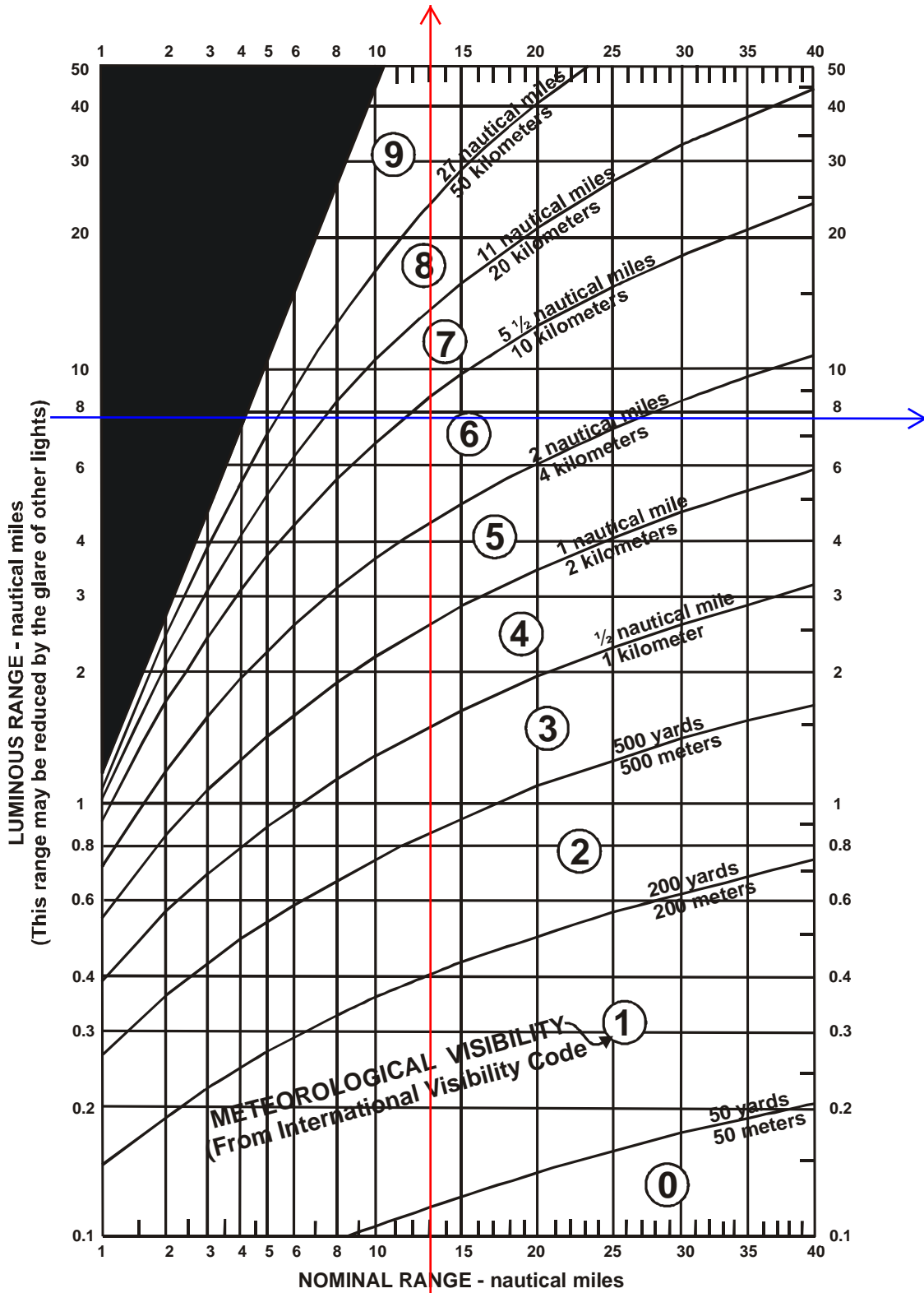
Luminous Range Diagram
